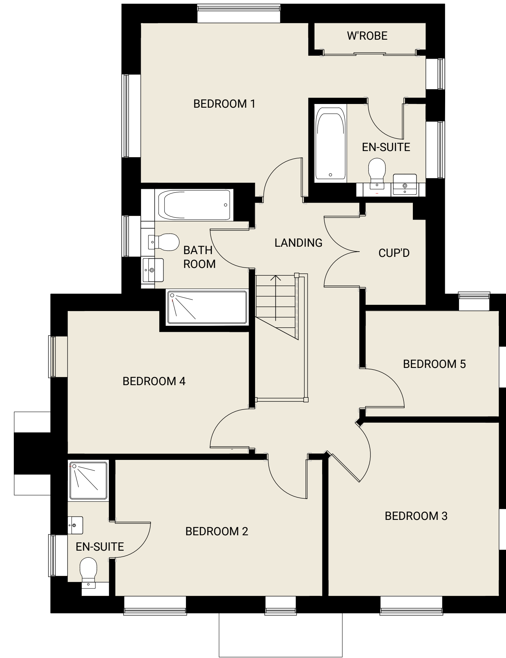
FIRST FLOOR
